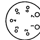
American Small 7 Pin (SM7)
